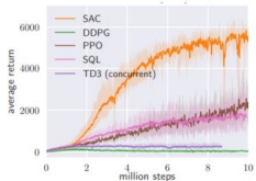
(f) Humanoid (rllab)
